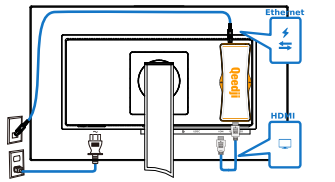
Configuration #3 - HDMI + Ethernet PoE
