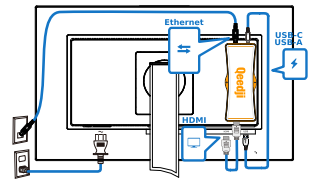
Configuration #4 - HDMI + Ethernet + USB
